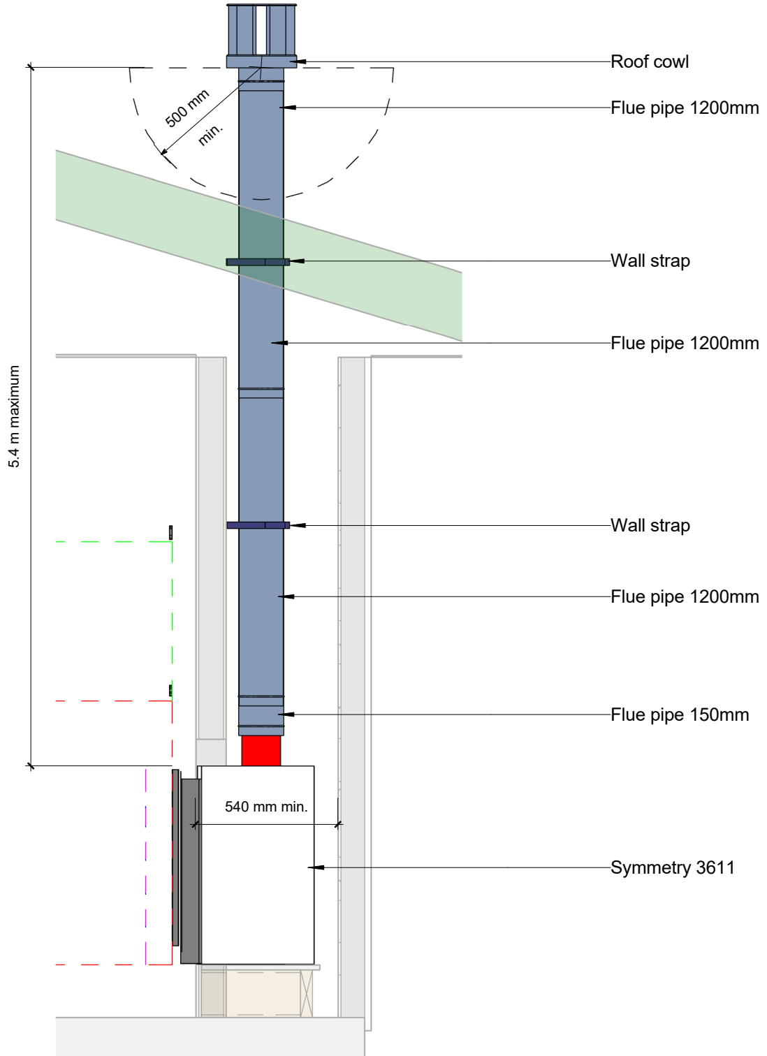
Section Across
